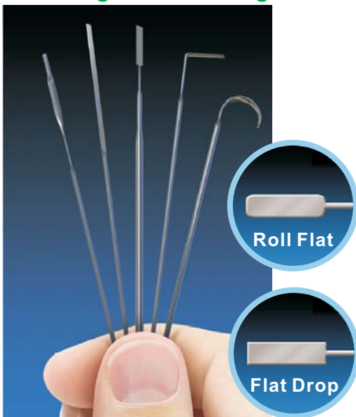
Samples of Pressed and Flattened Wire
